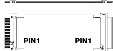
41 WAY FDC WITH DF-9 CONNECTOR
