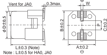
▨ : Dummy terminals
