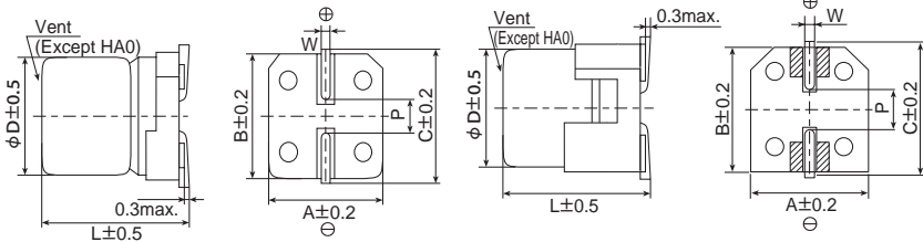
▨ : Dummy terminals
